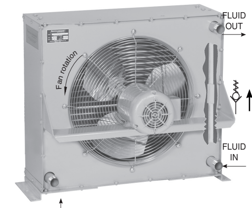
TWO PASS
